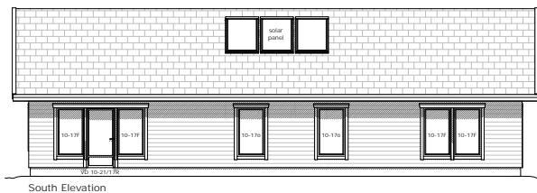
South Elevation
