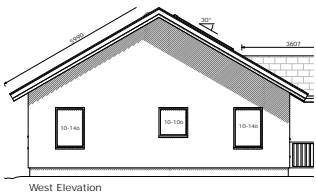
West Elevation
