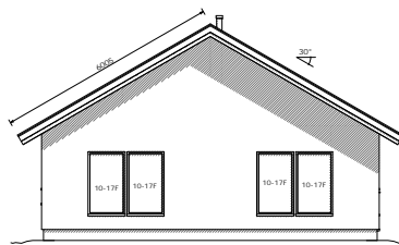
West Elevation
