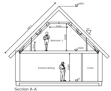
Section A-A Schematic section only - for dimensions and details please refer to the Standard section
