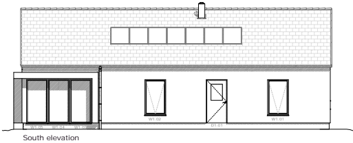
South elevation
