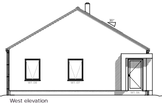
West elevation
