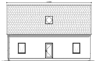
North elevation
