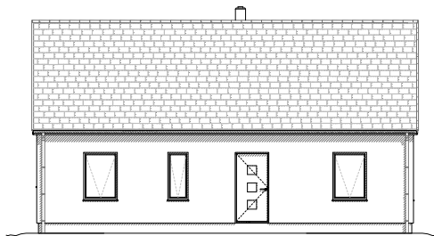
West Elevation
