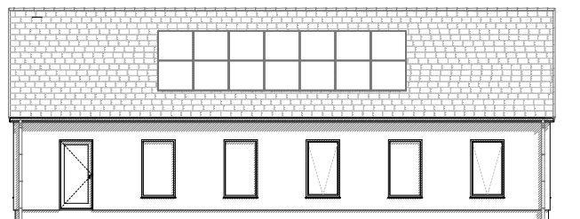
South Elevation
