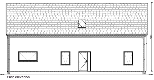
East elevation
