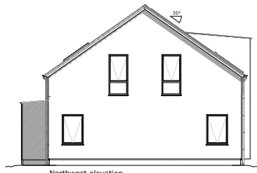
Northwest elevation
