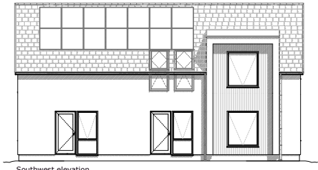
Southwest elevation
