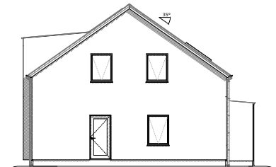
Southeast elevation
