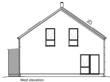
West elevation
