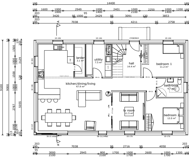
ground floor TUFA: 116.2 m 2
