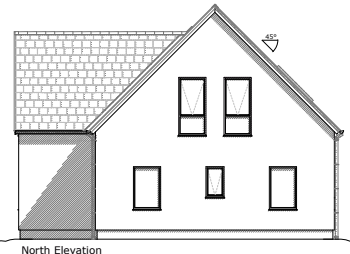
North Elevation
