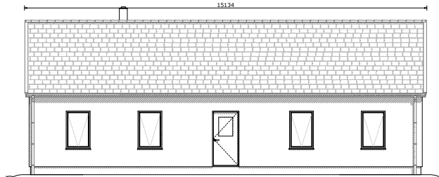
North Elevation
