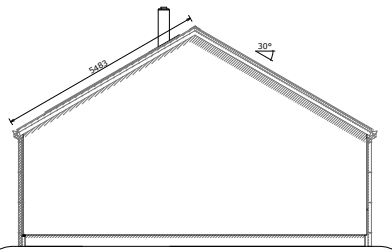
East Elevation
