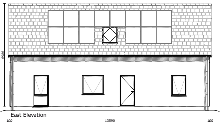
East Elevation
