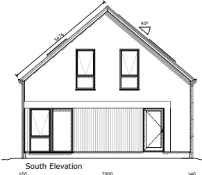
South Elevation
