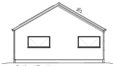
Southeast Elevation
