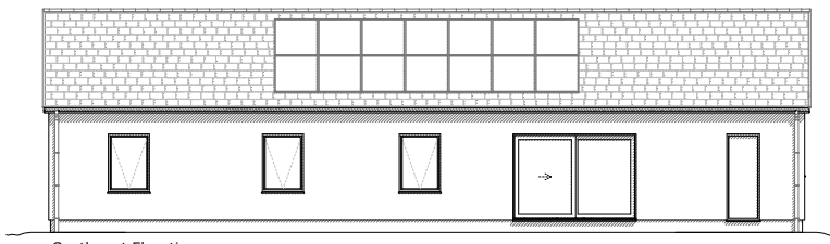
Southwest Elevation
