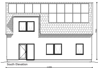
South Elevation
