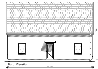
North Elevation
