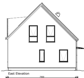
East Elevation
