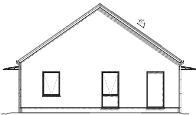
Southwest Elevation
