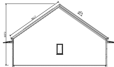
Northeast Elevation
