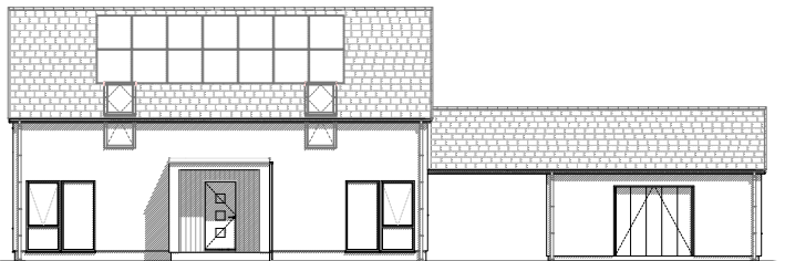
Southeast elevation
