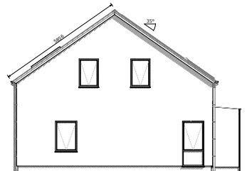
Southwest elevation
