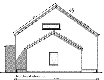
Northeast elevation
