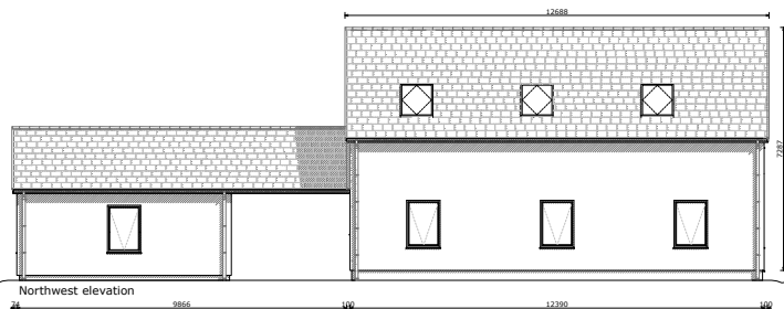
Northwest elevation
