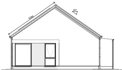
Southeast Elevation
