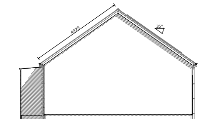
Northwest Elevation
