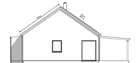
West Elevation
