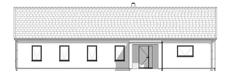
North Elevation
