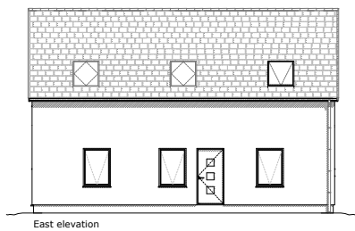
East elevation
