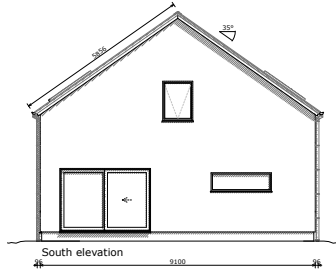
South elevation
