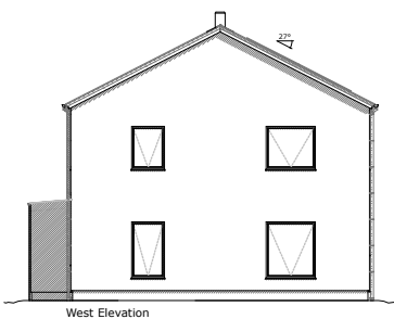
West Elevation
