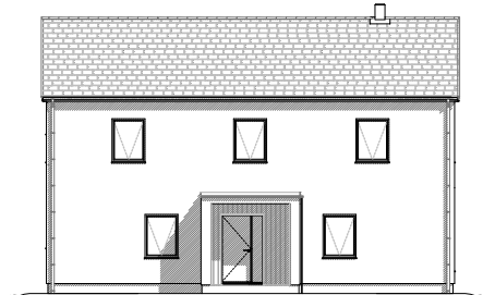
North Elevation
