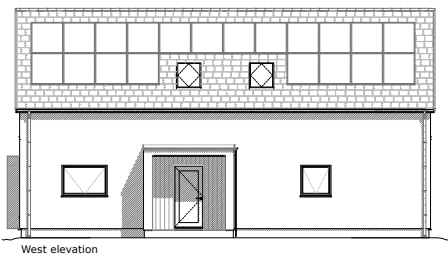
West elevation
