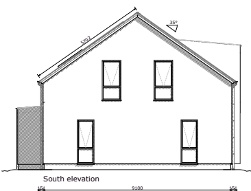
South elevation
