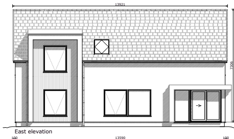
East elevation
