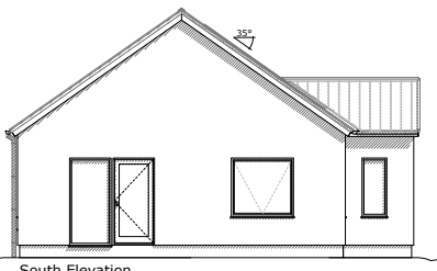
South Elevation
