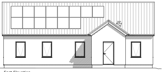
East Elevation
