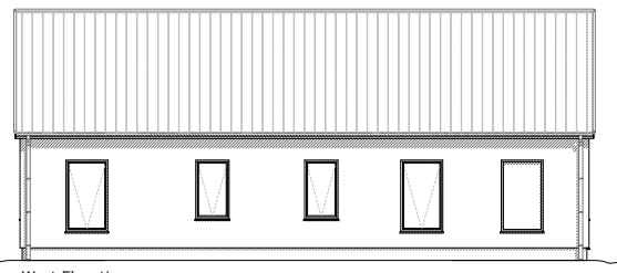
West Elevation
