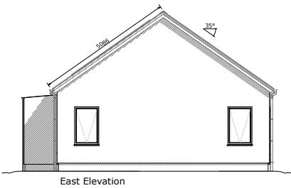
East Elevation
