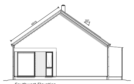
Southwest Elevation
