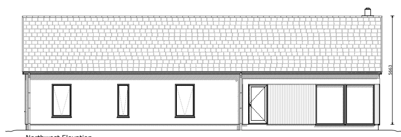
Northwest Elevation
