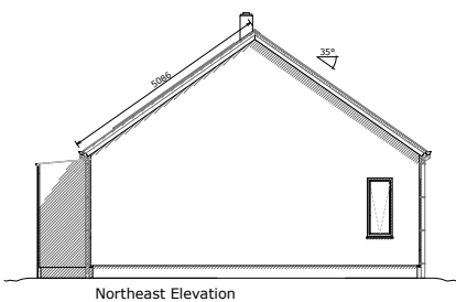
Northeast Elevation
