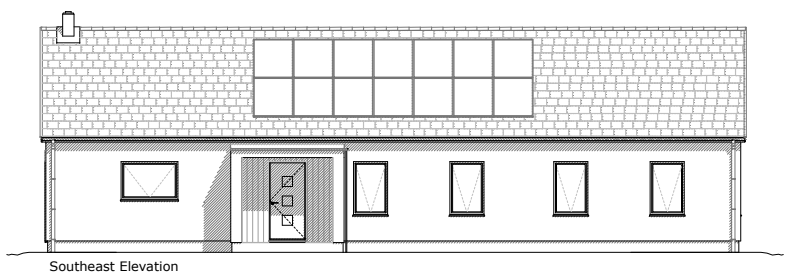
Southeast Elevation
