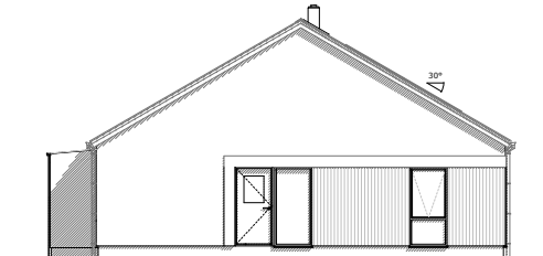
Northwest Elevation
