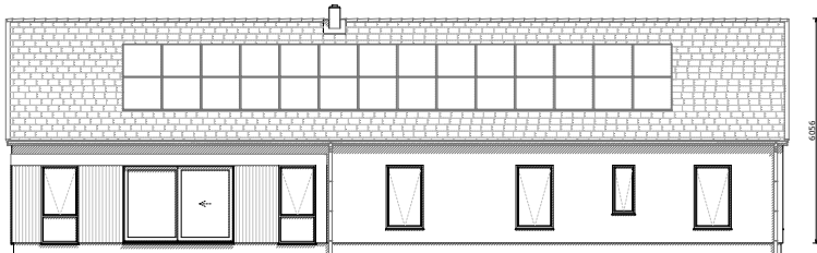
Southwest Elevation
