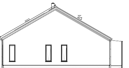
Southeast Elevation
